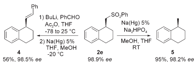
Scheme 2. Useful transformations of enantioenriched sulfones.
